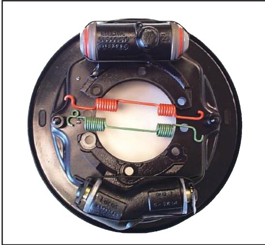
Backing Plate
